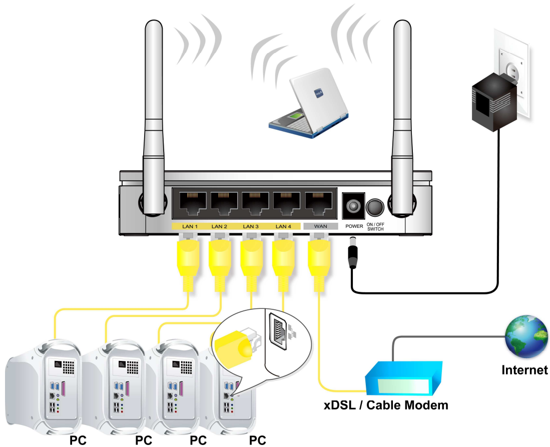
Figure 5: Overview of Hardware Connections
