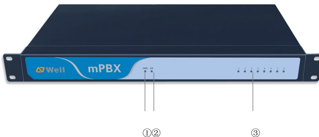
Figure 1-2 mPBX Pro Front Panel Picture
